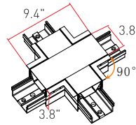
MAG38-CROSS Illuminated Cross Shape Joiner
