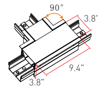
MAG38-T Illuminated T Shape Joiner
