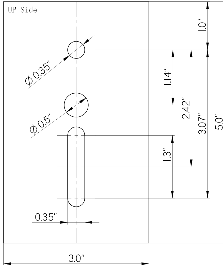
Side Arm mount Drill Pattern for EPT2
