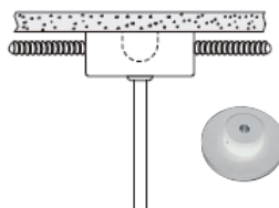
MELO-PMK-RS-SM-4-4FT-WH Rigid stem mount for 4" MELO, 4ft long stem, white (surface mounted junction box)
