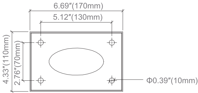
BASE PLATE
