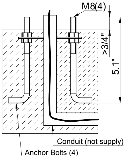
ANCHOR BOLTS
