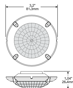
L7 Lens
