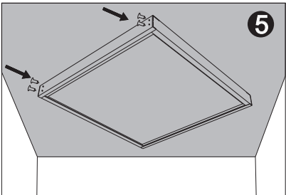
5. Fix the last frame with screw A.
