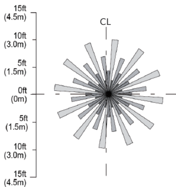
High Bay Lens - Top View at 8 ft(2.4m)
