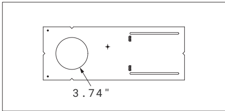
POR04-RIP-N Rough-in Plate. New Version
