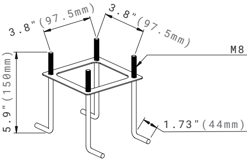
ANCHOR BOLTS
