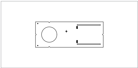
POR04-ADJ-RIP1 Rough-In Plate. New Construction. Pre-mounting Plate. Opening Ø4-1/4".
